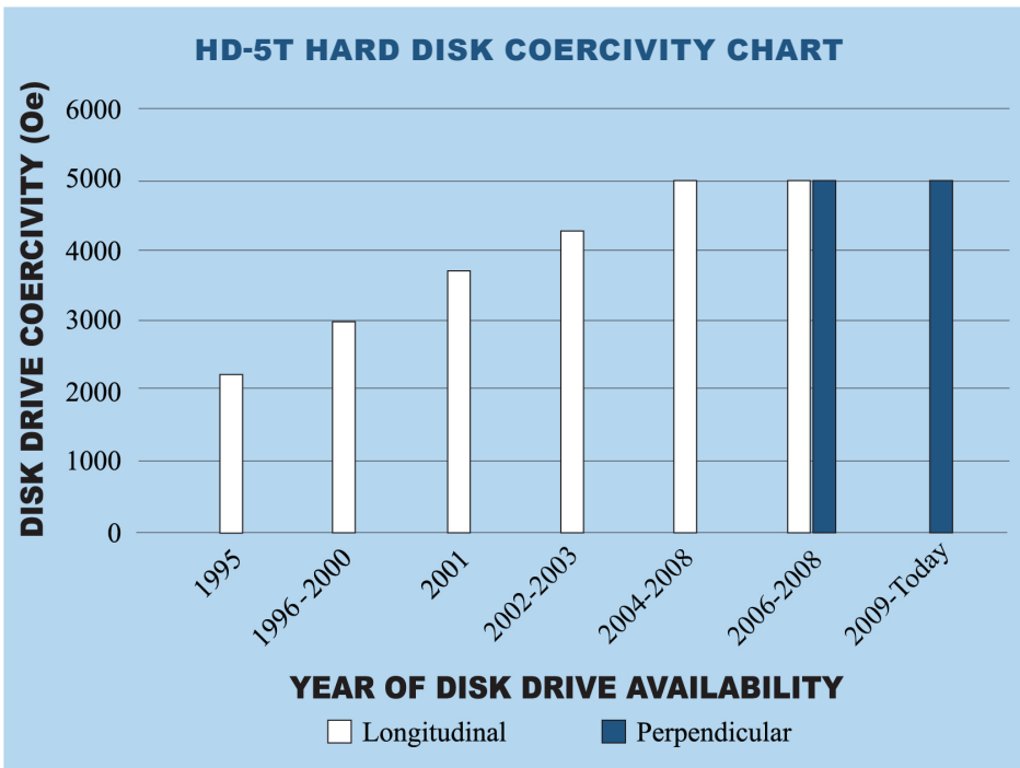
The HD-5T Degausser accommodates the following HDD form factors: 3.5 inch, 2.5 inch, 1.8 inch and smaller.
